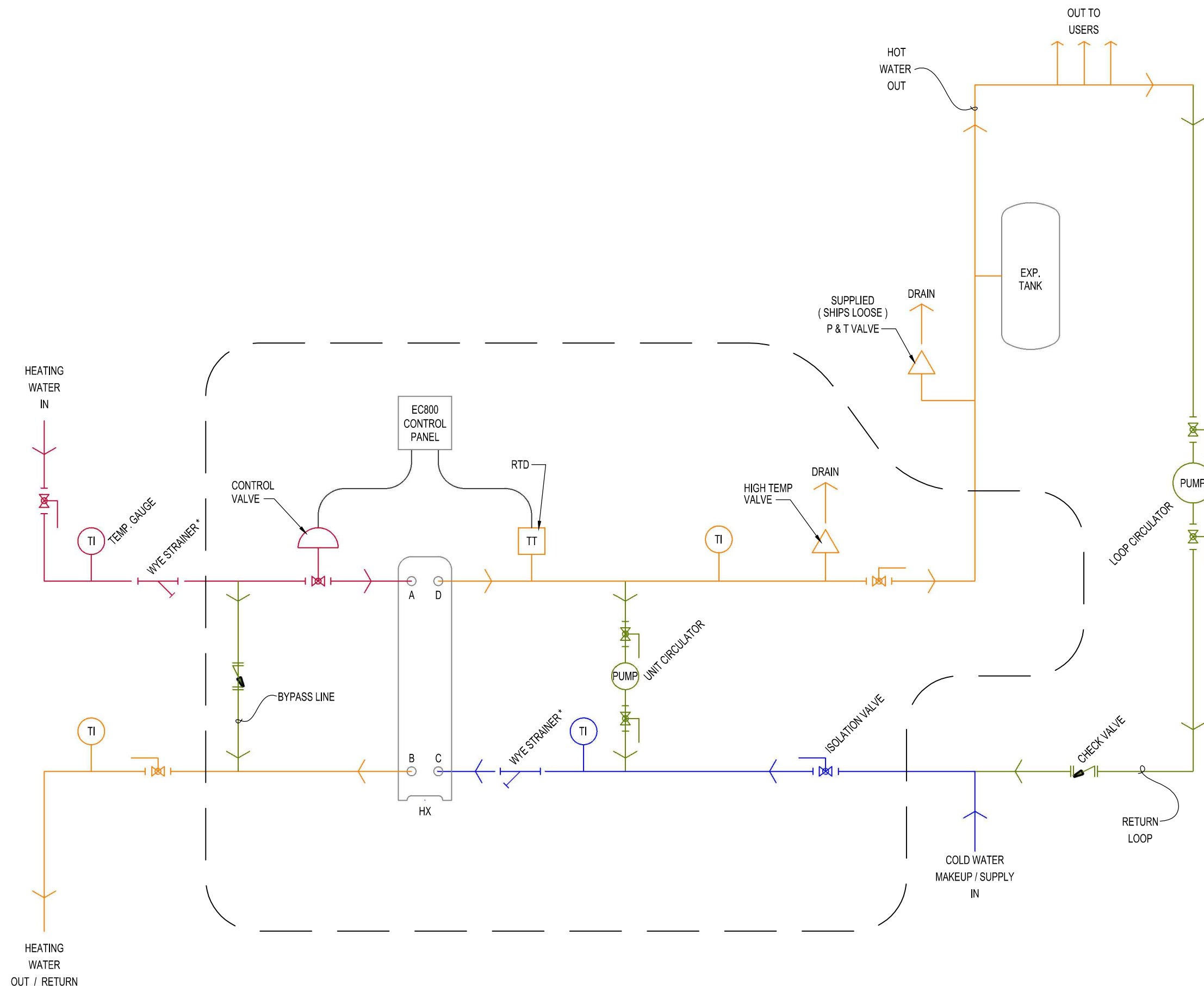
PLATE PAK SYSTEM CONNECTIONS & LAYOUT DIAGRAM
